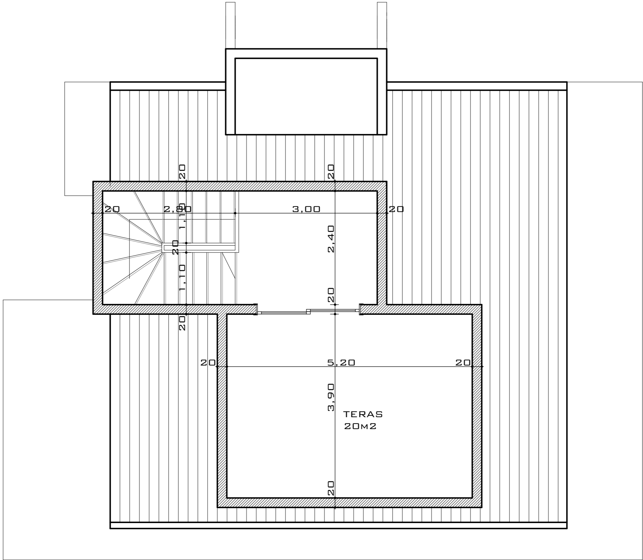
ÇATI KAT PLANI
